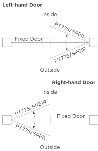
775 EXTENDED STRIKE PLATE PART NO. PT775/SPEILS
