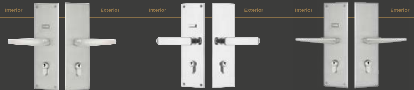
ROCHAS TRILOCK PART NO. 8904ROC Available finishes: SS ALLURE TRILOCK PART NO. 8904ALL Available finishes: SS / PS ENCHANT TRILOCK PART NO. 8904ENC Available finishes: SS
