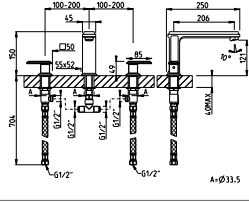
46045 three hole bath 46040 five hole bath
