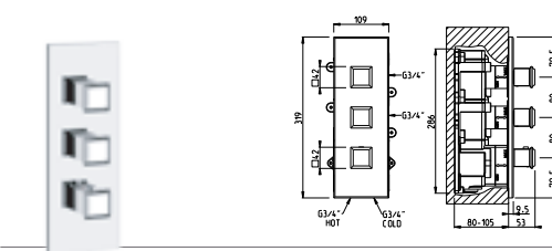
43103_46204 2 exits 43105_46206 3 exits 43107_46208 4 exits 43109_46210 5 exits 43111_46212 3 exits with diverter
