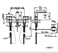
WITH WHITE/BLACK INSERT 46015 46014 without waste
