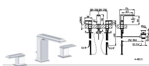
WITH WHITE/BLACK INSERT 46015 46014 without waste
