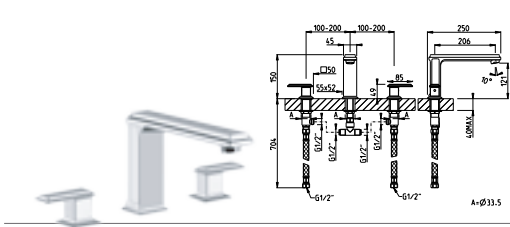
46045 three hole bath 46040 five hole bath
