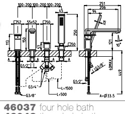
46037 four hole bath 46043 three hole bath 46047 two hole bath
