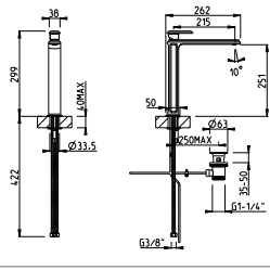
WITH WHITE/BLACK INSERT 46009 46008 without waste
