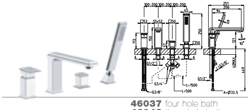
46037 four hole bath 46043 three hole bath 46047 two hole bath
